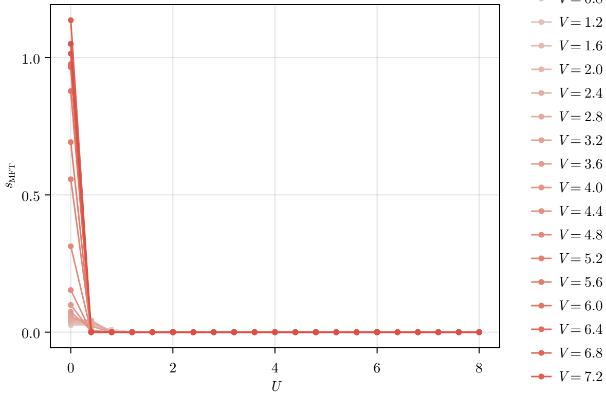
s_{\text{MFT}} (t=1.0, L=256, \delta=0.0, \beta=100.0)
